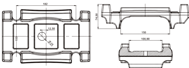
LOWER CAP 100MM
