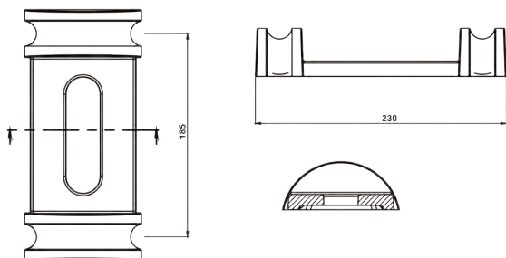
UPPER CAP 100MM
