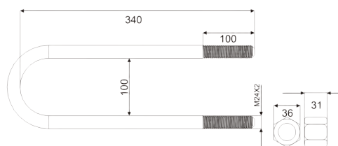
U BOLT W/NUTS
